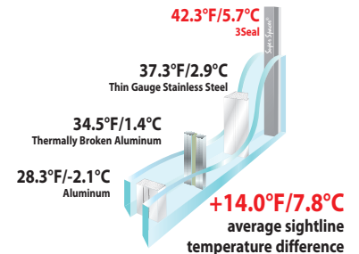
Thermal Conductivity Chart
